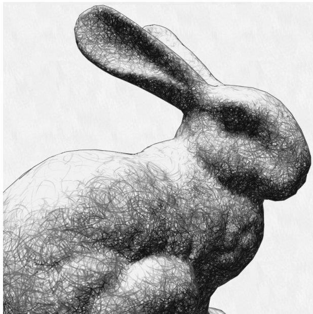
Figure 1: Bunny rendered using color volume texture; globe rendered using threshold textures (modulated per-pixel).
